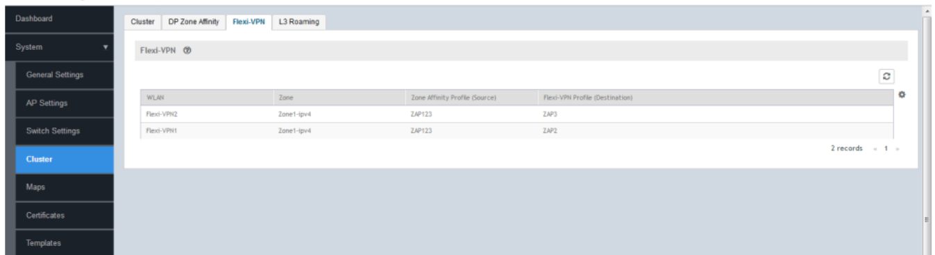
FIGURE 81 Enabling Flexi-VPN
