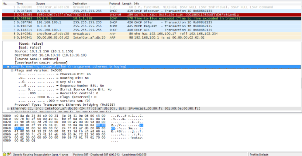
FIGURE 361 Example of SoftGRE packet format
